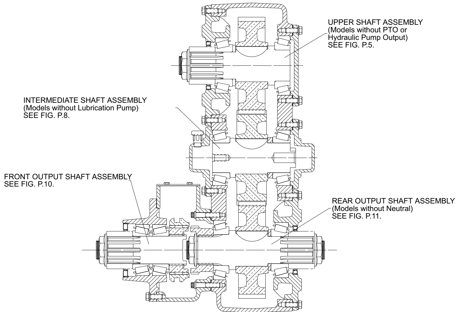
FIG P.1 - TYPICAL TC-170 BASIC TRANSFER CASE
