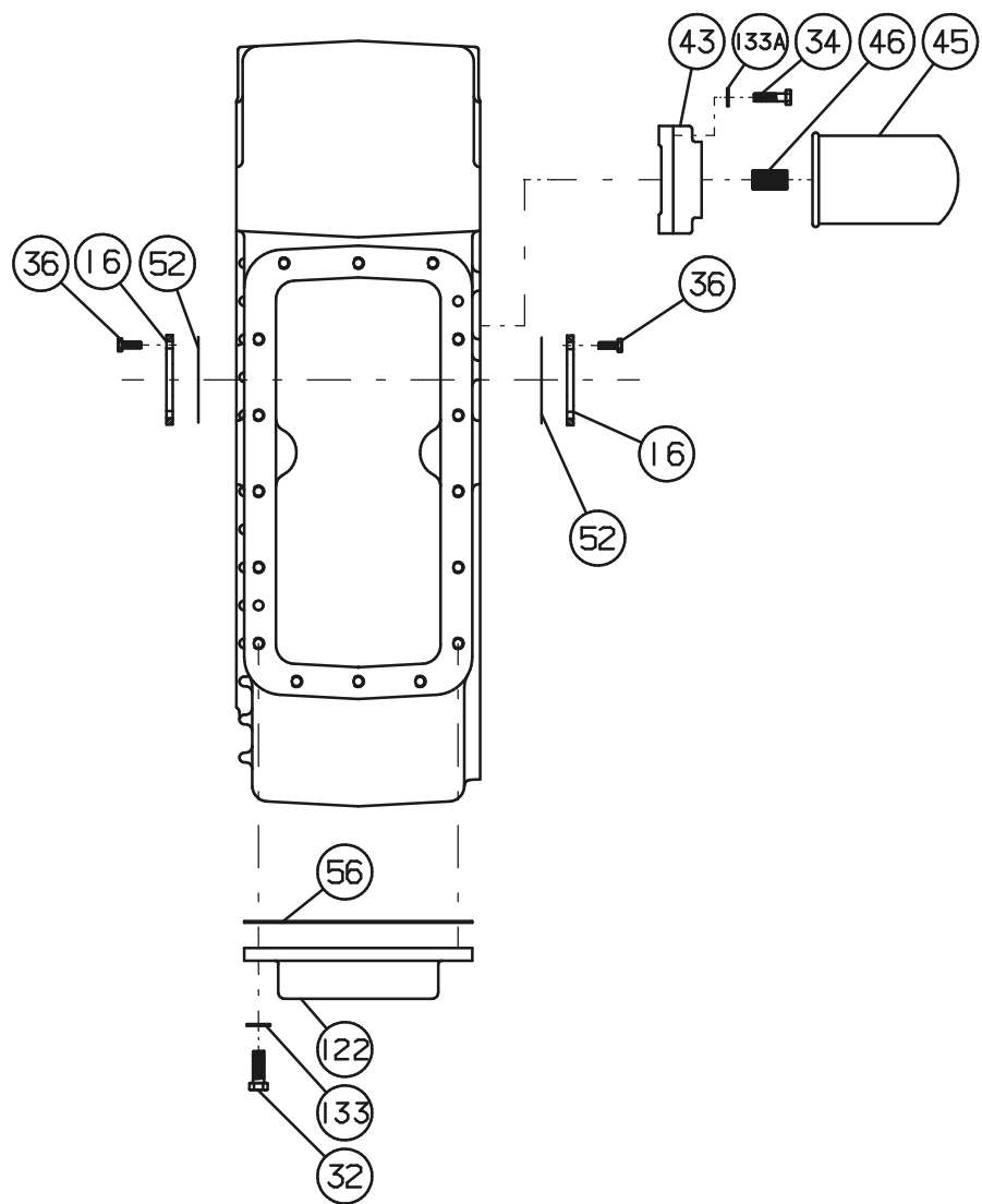
TC-143 CASE HOUSING PARTS 873-0031-006
