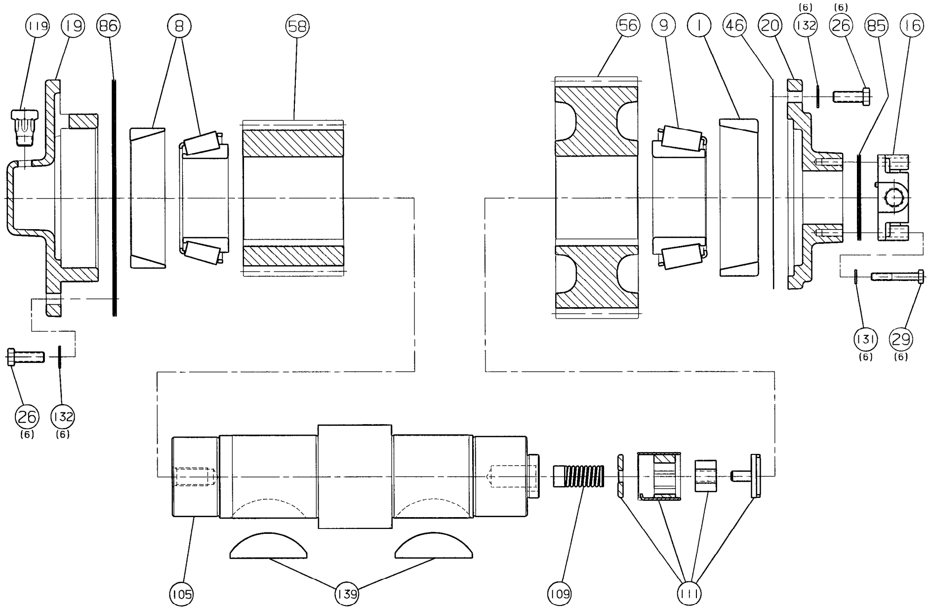
FIGURE 8.2 , TC-142 , INTERMEDIATE SHAFT PARTS
