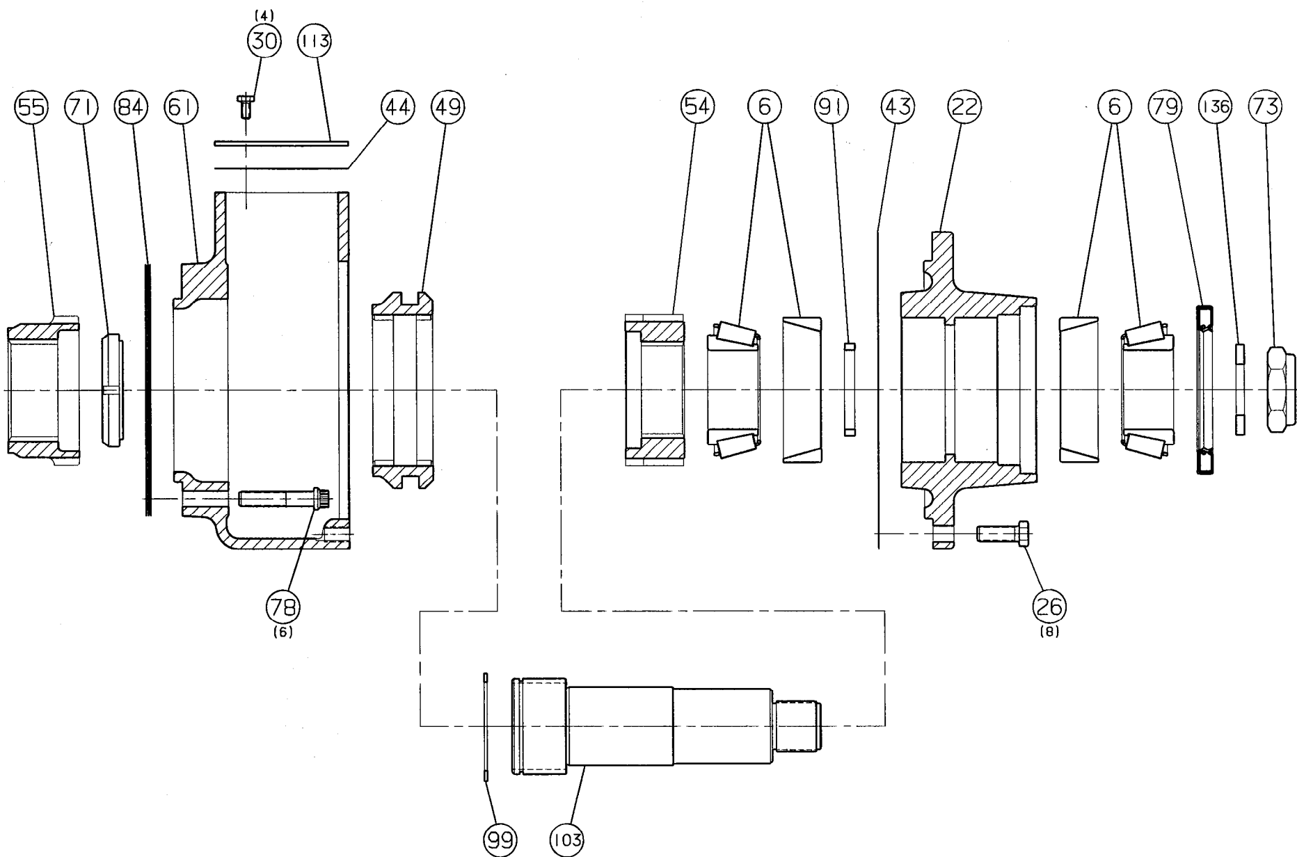
FIGURE 8.7 , TC-142 & TC-1421 , PTO OUTPUT SHAFT PARTS
