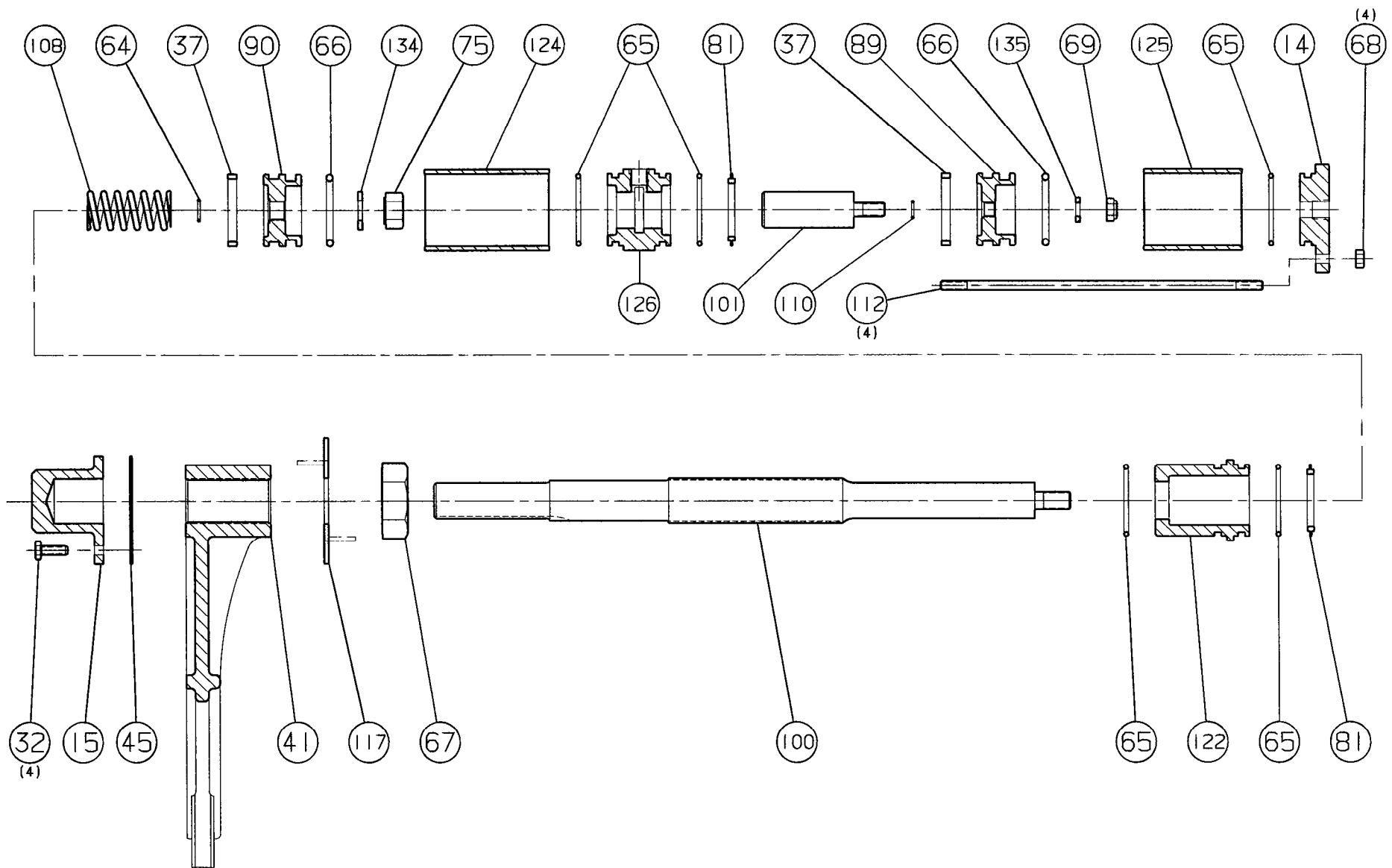
FIGURE 8.11 , TC-142 , AIR SHIFT CYLINDER PARTS FOR DIRECT , NEUTRAL & UNDERDRIVE
