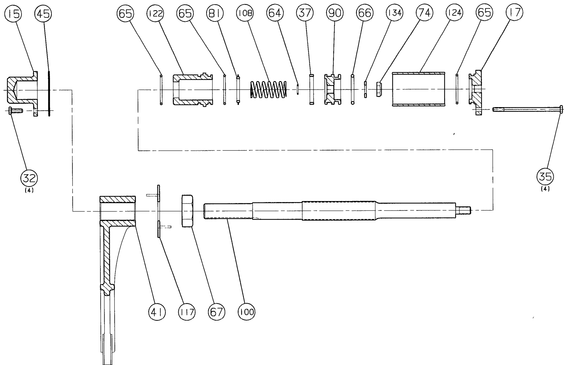
FIGURE 8.12 , TC-1421 , AIR SHIFT CYLINDER PARTS FOR DIRECT & NEUTRAL
